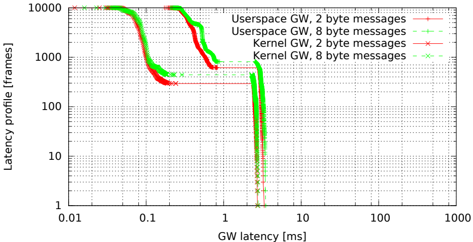
Kernel vs. userspace GW, no modifications (GW kernel 2.6.36.2-00015-g4f1bc4e, Traffic oneatatime, Load eth)
