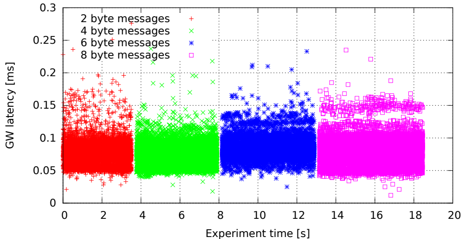
Single GW rule for all messages, no modifications (GW kernel 2.6.36.2-00015-g4f1bc4e, Traffic oneatatime, Load eth)
