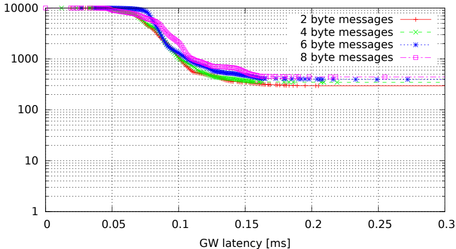
Single GW rule for all messages, no modifications, high (soft)irq task priority (GW kernel 2.6.36.2-00015-g4f1bc4e, Traffic onetatime, Load eth)
