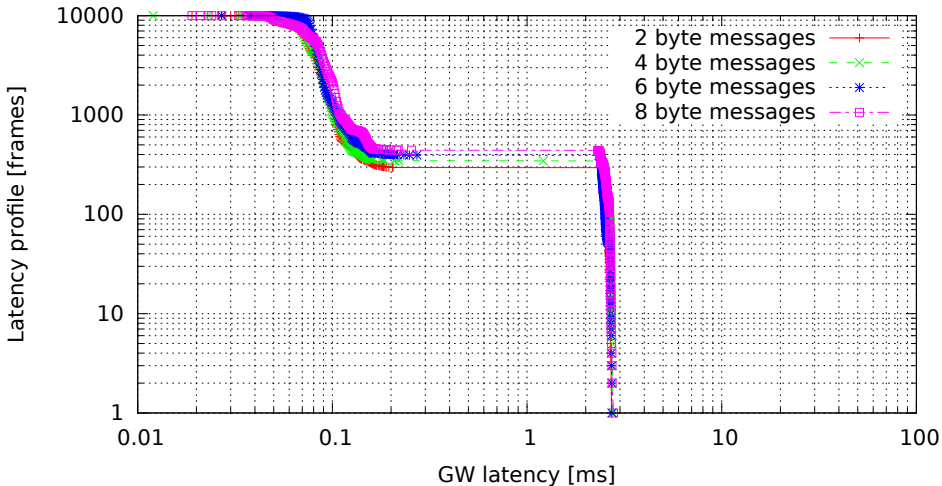
Single GW rule for all messages, no modifications, high (soft)irq task priority (GW kernel 2.6.36.2-00015-g4f1bc4e, Traffic onetatime, Load eth)
