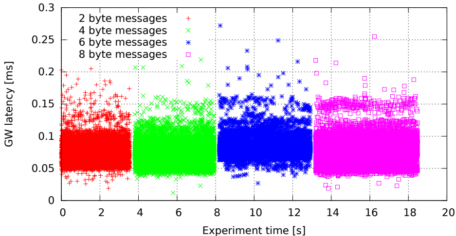
Single GW rule for all messages, no modifications, high (soft)irq task priority (GW kernel 2.6.36.2-00015-g4f1bc4e, Traffic oneatatime, Load eth)
