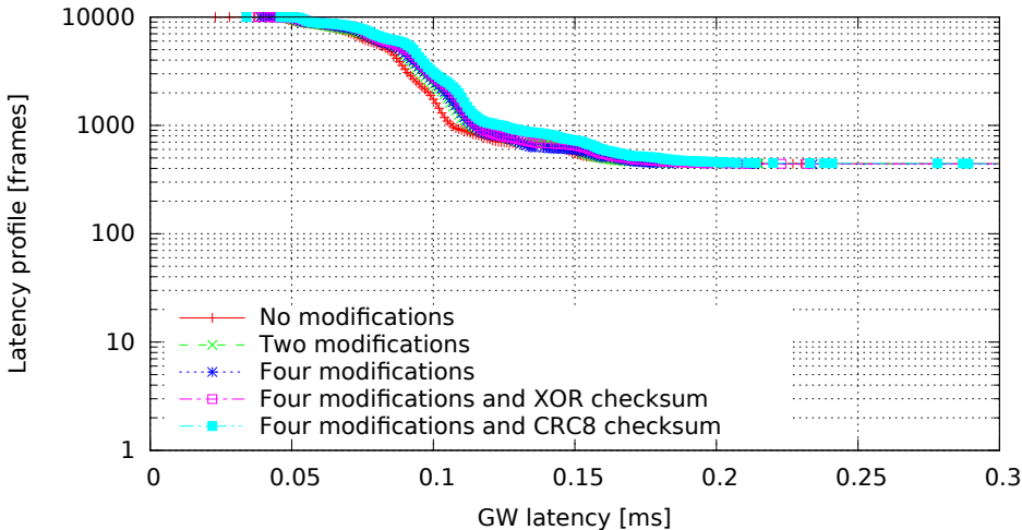
Single GW rule for all messages with modifications, 8 byte messages (GW kernel 2.6.36.2-00015-g4f1bc4e, Traffic onetatime, Load eth)
