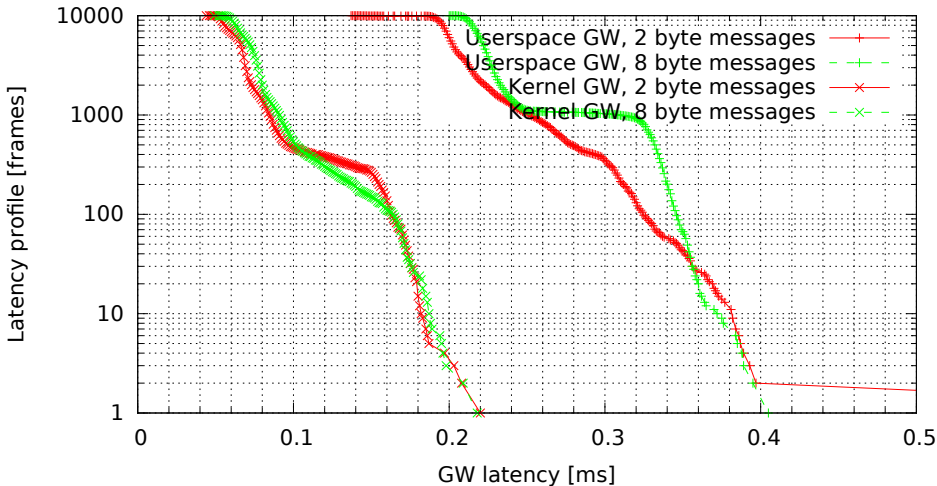
Kernel vs. userspace GW, no modifications (GW kernel 2.6.36.2-00015-g4f1bc4e, Traffic oneatatime, Load cpu)
