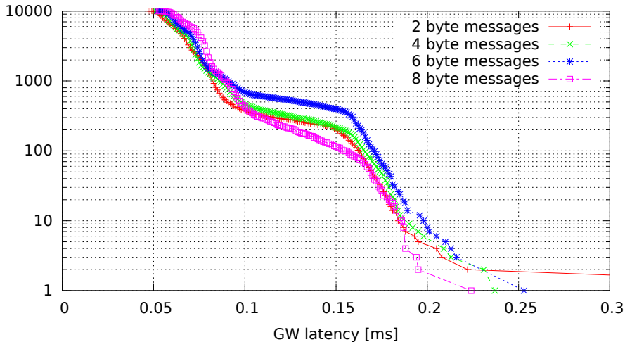
Single GW rule for all messages, no modifications (GW kernel 2.6.36.2-00015-g4f1bc4e, Traffic oneatatime, Load cpu)
