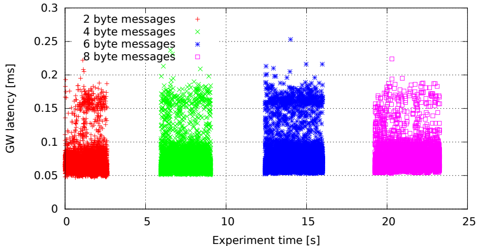
Single GW rule for all messages, no modifications (GW kernel 2.6.36.2-00015-g4f1bc4e, Traffic oneatatime, Load cpu)
