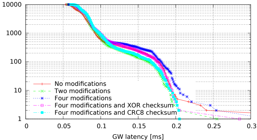
Single GW rule for all messages with modifications, 8 byte messages (GW kernel 2.6.36.2-00015-g4f1bc4e, Traffic oneatatime, Load cpu)
