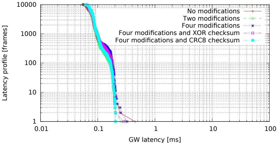
Single GW rule for all messages with modifications, 8 byte messages (GW kernel 2.6.36.2-00015-g4f1bc4e, Traffic oneatatime, Load cpu)
