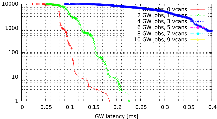
Chained GWs on multiple VCAN interfaces (GW kernel 2.6.36.2-00015-g4f1bc4e, Traffic flood, Load none)
