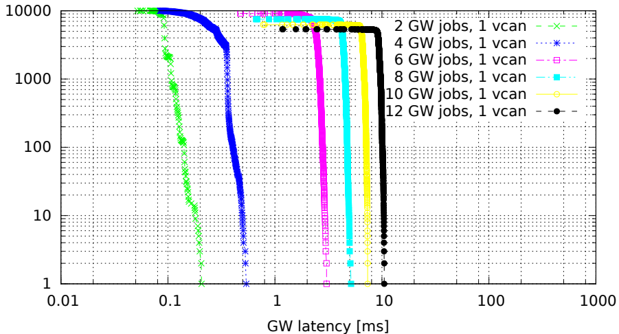
Chained GWs on a single VCAN interface (GW kernel 2.6.36.2-00015-g4f1bc4e, Traffic flood, Load none)
