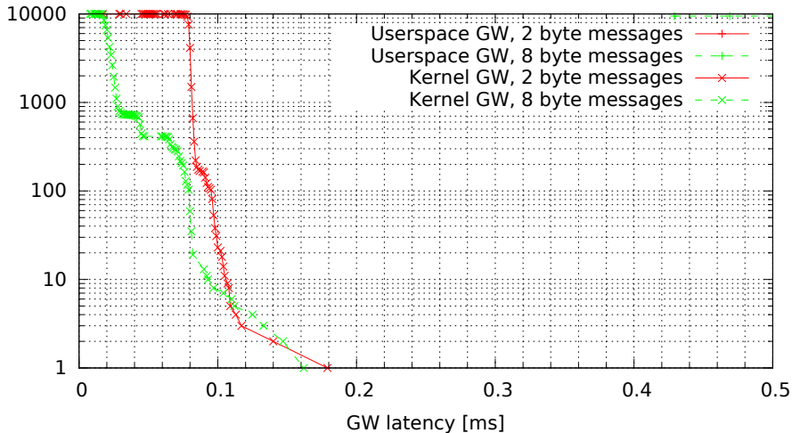
Kernel vs. userspace GW, no modifications (GW kernel 2.6.36.2-00015-g4f1bc4e, Traffic flood, Load none)
