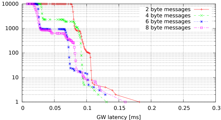
Single GW rule for all messages, no modifications (GW kernel 2.6.36.2-00015-g4f1bc4e, Traffic flood, Load none)
