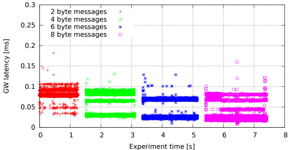
Single GW rule for all messages, no modifications (GW kernel 2.6.36.2-00015-g4f1bc4e, Traffic flood, Load none)
