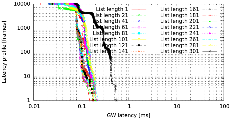
Different lengths of filter list, only the last one matches (GW kernel 2.6.36.2-00015-g4f1bc4e, Traffic flood, Load none)
