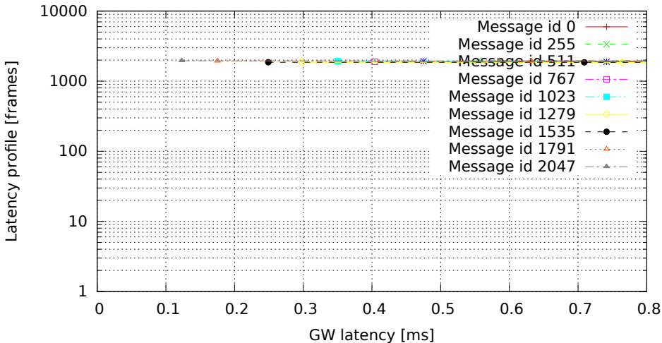
2048 GW rules (one per id, mask 0x7FF), no modifications (GW kernel 2.6.36.2-00015-g4f1bc4e, Traffic flood, Load none)
