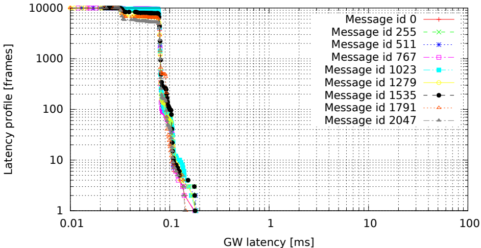
2048 GW rules (one per id, mask C00007FF), no modifications (GW kernel 2.6.36.2-00015-g4f1bc4e, Traffic flood, Load none)
