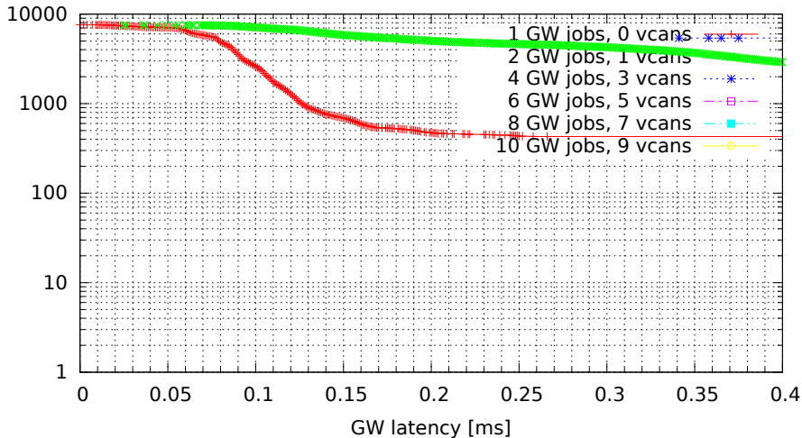
Chained GWs on multiple VCAN interfaces (GW kernel 2.6.36.2-00015-g4f1bc4e, Traffic flood, Load eth)
