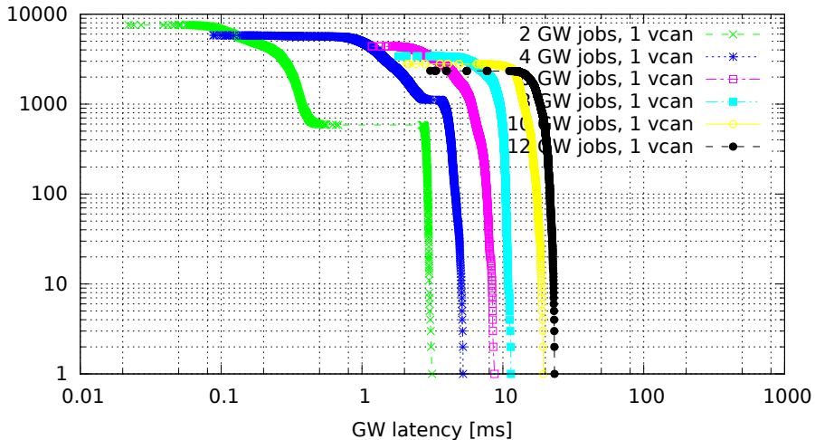
Chained GWs on a single VCAN interface (GW kernel 2.6.36.2-00015-g4f1bc4e, Traffic flood, Load eth)
