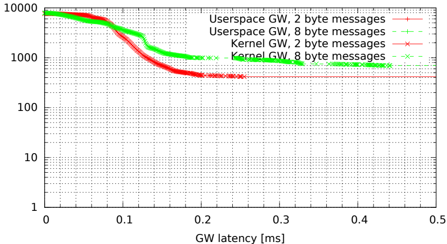
Kernel vs. userspace GW, no modifications (GW kernel 2.6.36.2-00015-g4f1bc4e, Traffic flood, Load eth)
