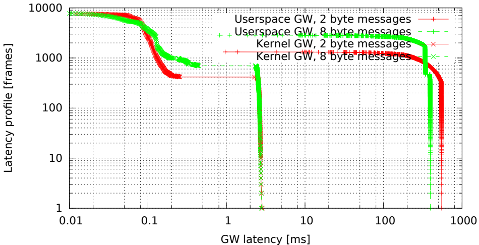
Kernel vs. userspace GW, no modifications (GW kernel 2.6.36.2-00015-g4f1bc4e, Traffic flood, Load eth)
