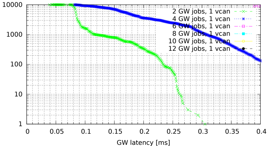
Chained GWs on a single VCAN interface (GW kernel 2.6.36.2-00015-g4f1bc4e, Traffic flood, Load cpu)
