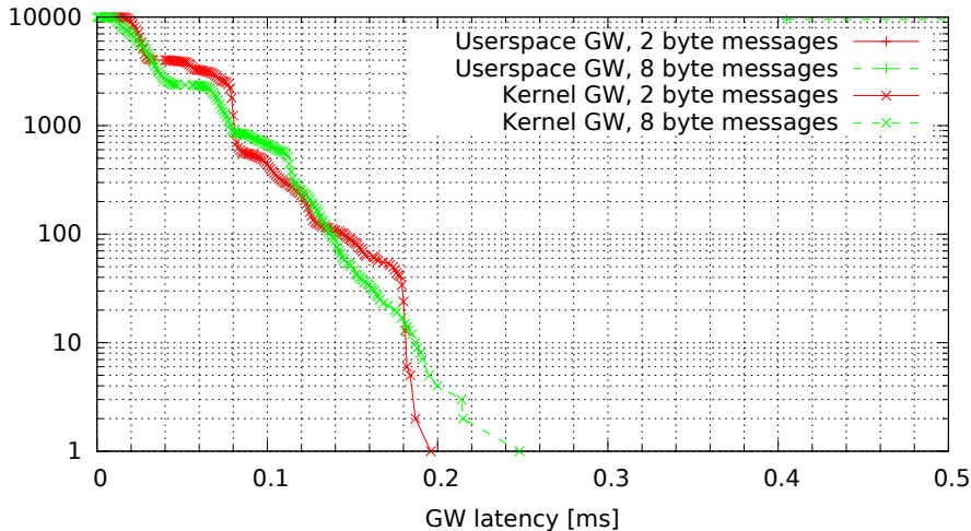
Kernel vs. userspace GW, no modifications (GW kernel 2.6.36.2-00015-g4f1bc4e, Traffic flood, Load cpu)
