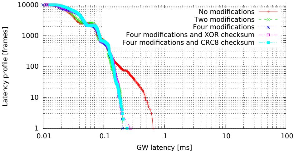
Single GW rule for all messages with modifications, 8 byte messages (GW kernel 2.6.36.2-00015-g4f1bc4e, Traffic flood, Load cpu)
