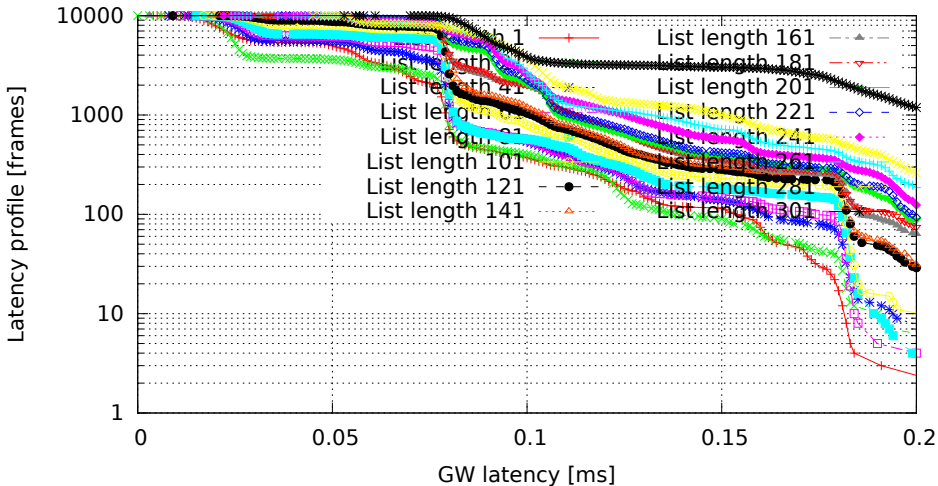
Different lengths of filter list, only the last one matches (GW kernel 2.6.36.2-00015-g4f1bc4e, Traffic flood, Load cpu)
