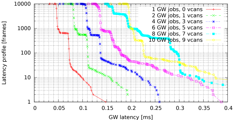
Chained GWs on multiple VCAN interfaces (GW kernel 2.6.36.2-00015-g4f1bc4e, Traffic 50, Load none)
