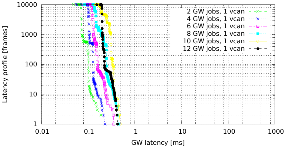
Chained GWs on a single VCAN interface (GW kernel 2.6.36.2-00015-g4f1bc4e, Traffic 50, Load none)
