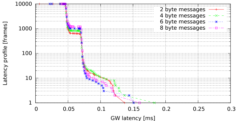
Single GW rule for all messages, no modifications (GW kernel 2.6.36.2-00015-g4f1bc4e, Traffic 50, Load none)
