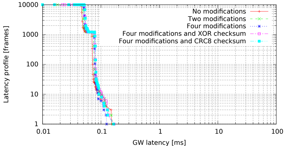
Single GW rule for all messages with modifications, 8 byte messages (GW kernel 2.6.36.2-00015-g4f1bc4e, Traffic 50, Load none)
