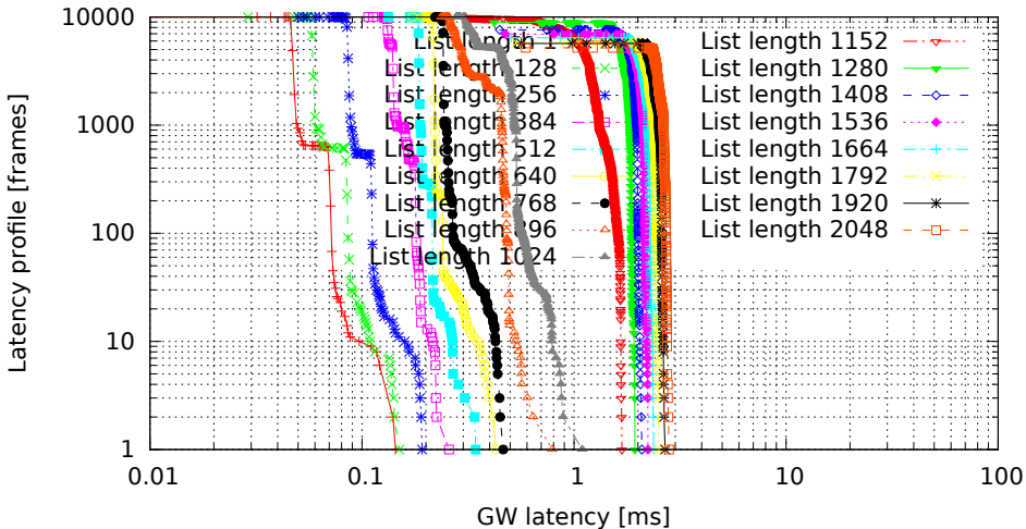
Different lengths of filter list, only the last one matches (GW kernel 2.6.36.2-00015-g4f1bc4e, Traffic 50, Load none)
