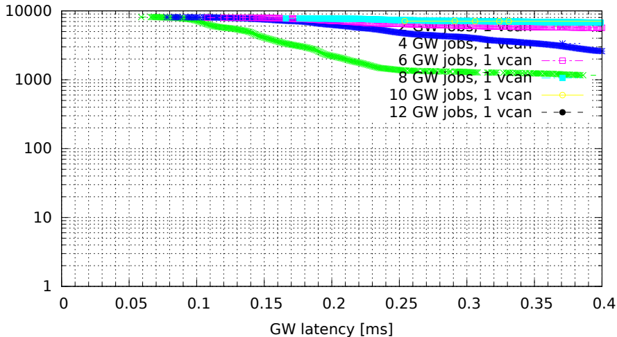
Chained GWs on a single VCAN interface (GW kernel 2.6.36.2-00015-g4f1bc4e, Traffic 50, Load eth)
