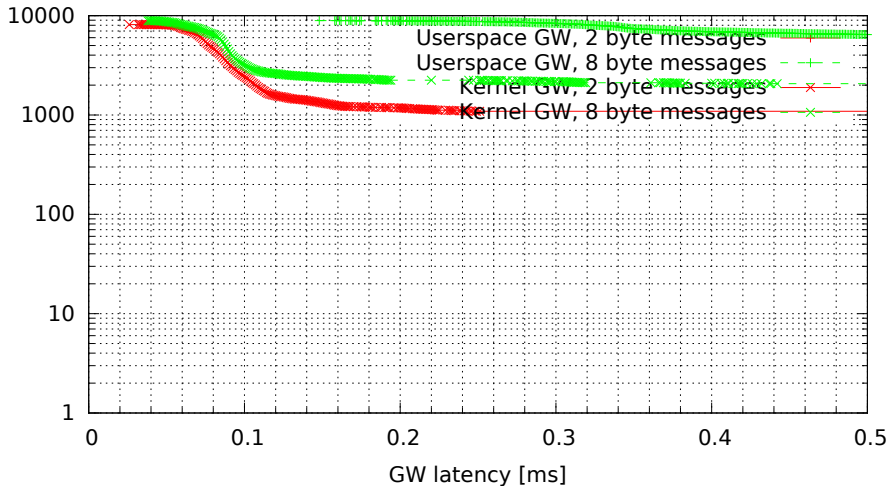
Kernel vs. userspace GW, no modifications (GW kernel 2.6.36.2-00015-g4f1bc4e, Traffic 50, Load eth)
