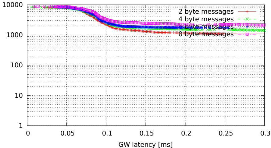
Single GW rule for all messages, no modifications (GW kernel 2.6.36.2-00015-g4f1bc4e, Traffic 50, Load eth)
