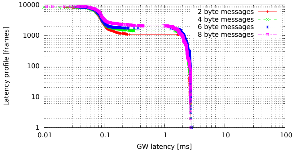
Single GW rule for all messages, no modifications (GW kernel 2.6.36.2-00015-g4f1bc4e, Traffic 50, Load eth)
