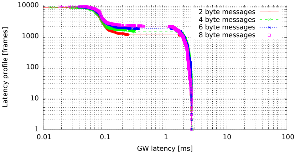
Single GW rule for all messages, no modifications, high (soft)irq task priority (GW kernel 2.6.36.2-00015-g4f1bc4e, Traffic 50, Load eth)
