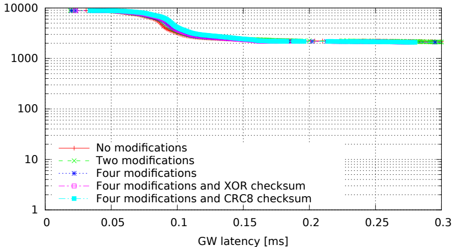
Single GW rule for all messages with modifications, 8 byte messages (GW kernel 2.6.36.2-00015-g4f1bc4e, Traffic 50, Load eth)
