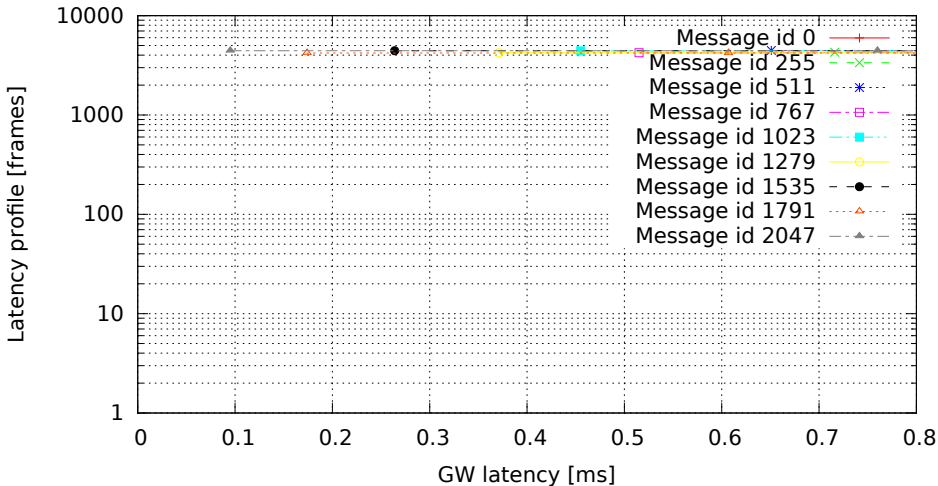
2048 GW rules (one per id, mask 0x7FF), no modifications (GW kernel 2.6.36.2-00015-g4f1bc4e, Traffic 50, Load eth)
