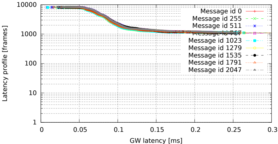
2048 GW rules (one per id, mask C00007FF), no modifications (GW kernel 2.6.36.2-00015-g4f1bc4e, Traffic 50, Load eth)
