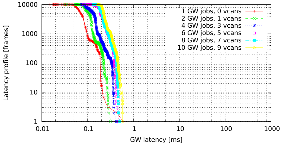
Chained GWs on multiple VCAN interfaces (GW kernel 2.6.36.2-00015-g4f1bc4e, Traffic 50, Load cpu)
