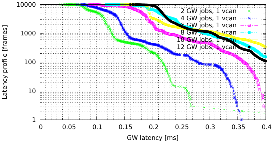
Chained GWs on a single VCAN interface (GW kernel 2.6.36.2-00015-g4f1bc4e, Traffic 50, Load cpu)
