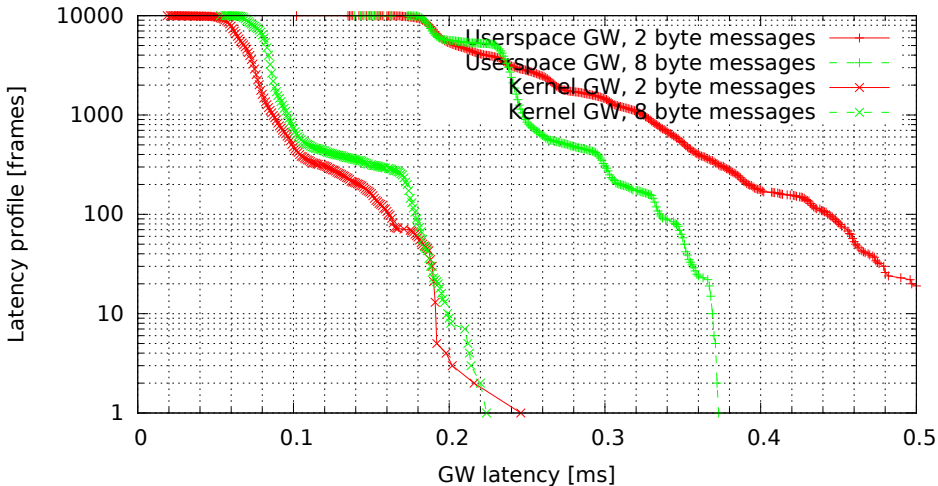
Kernel vs. userspace GW, no modifications (GW kernel 2.6.36.2-00015-g4f1bc4e, Traffic 50, Load cpu)
