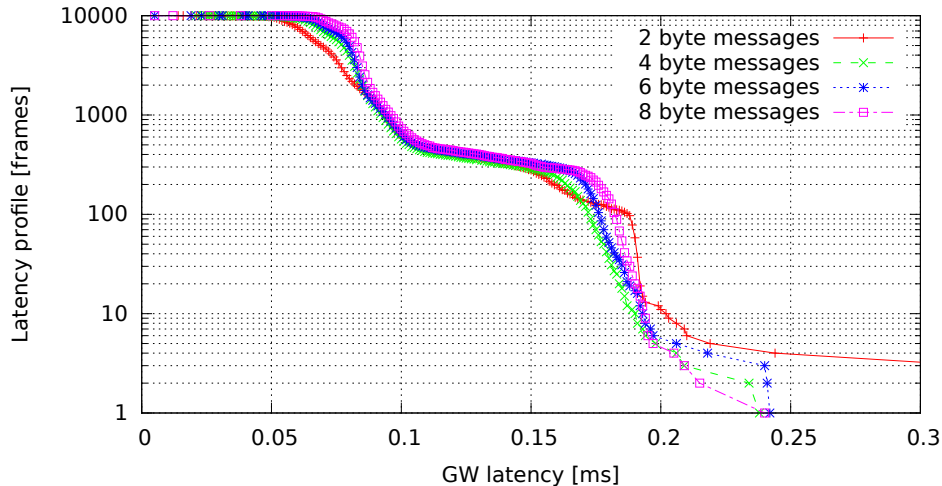
Single GW rule for all messages, no modifications (GW kernel 2.6.36.2-00015-g4f1bc4e, Traffic 50, Load cpu)
