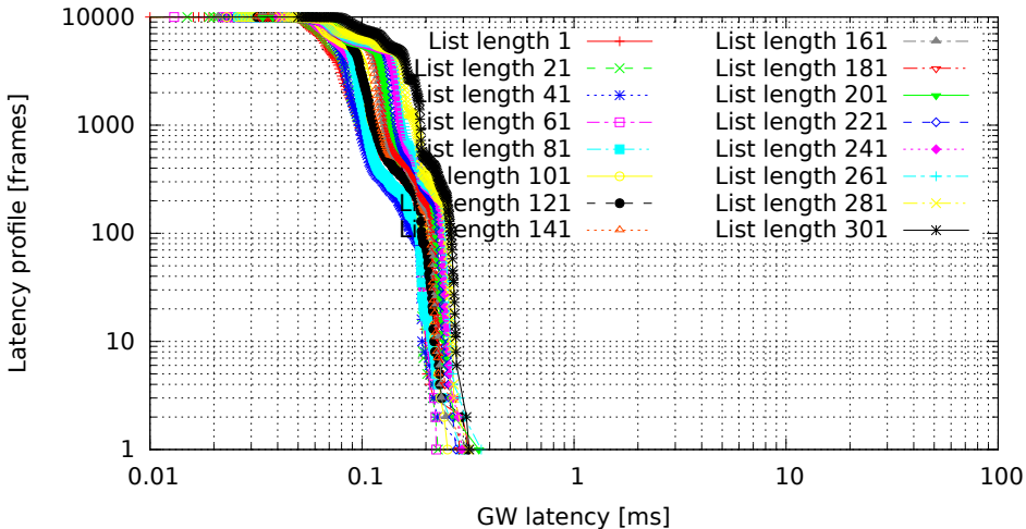
Different lengths of filter list, only the last one matches (GW kernel 2.6.36.2-00015-g4f1bc4e, Traffic 50, Load cpu)
