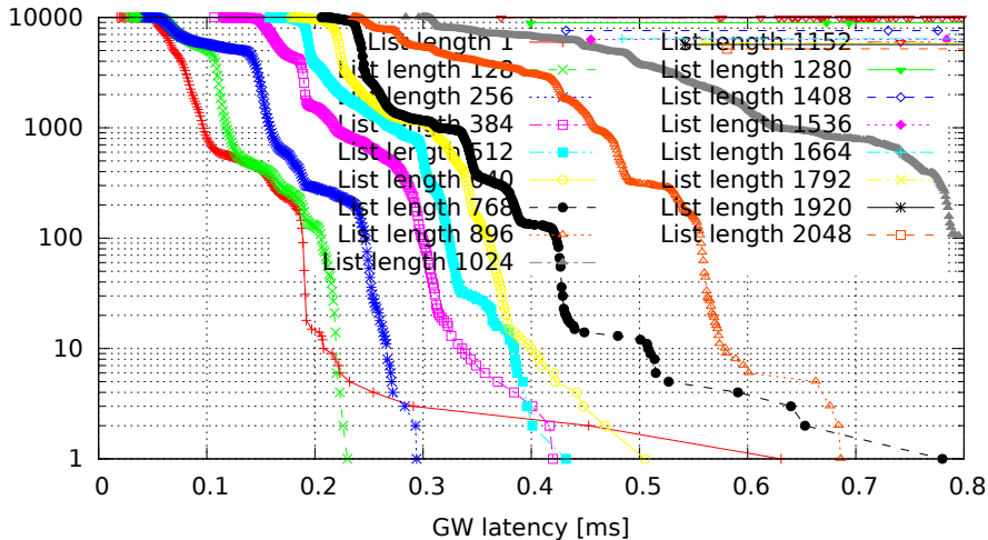
Different lengths of filter list, only the last one matches (GW kernel 2.6.36.2-00015-g4f1bc4e, Traffic 50, Load cpu)
