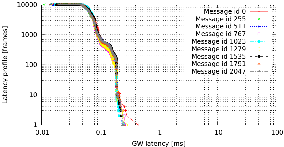
2048 GW rules (one per id, mask C00007FF), no modifications (GW kernel 2.6.36.2-00015-g4f1bc4e, Traffic 50, Load cpu)
