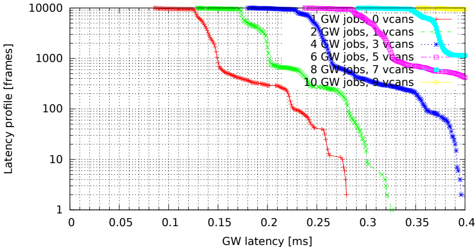
Chained GWs on multiple VCAN interfaces (GW kernel 2.6.33.7-rt29-00004-g92487e4, Traffic oneatatime, Load none)
