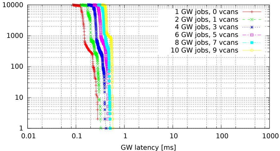
Chained GWs on multiple VCAN interfaces (GW kernel 2.6.33.7-rt29-00004-g92487e4, Traffic oneatatime, Load none)
