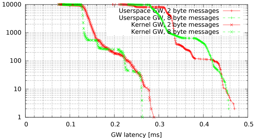
Kernel vs. userspace GW, no modifications (GW kernel 2.6.33.7-rt29-00004-g92487e4, Traffic oneatatime, Load none)
